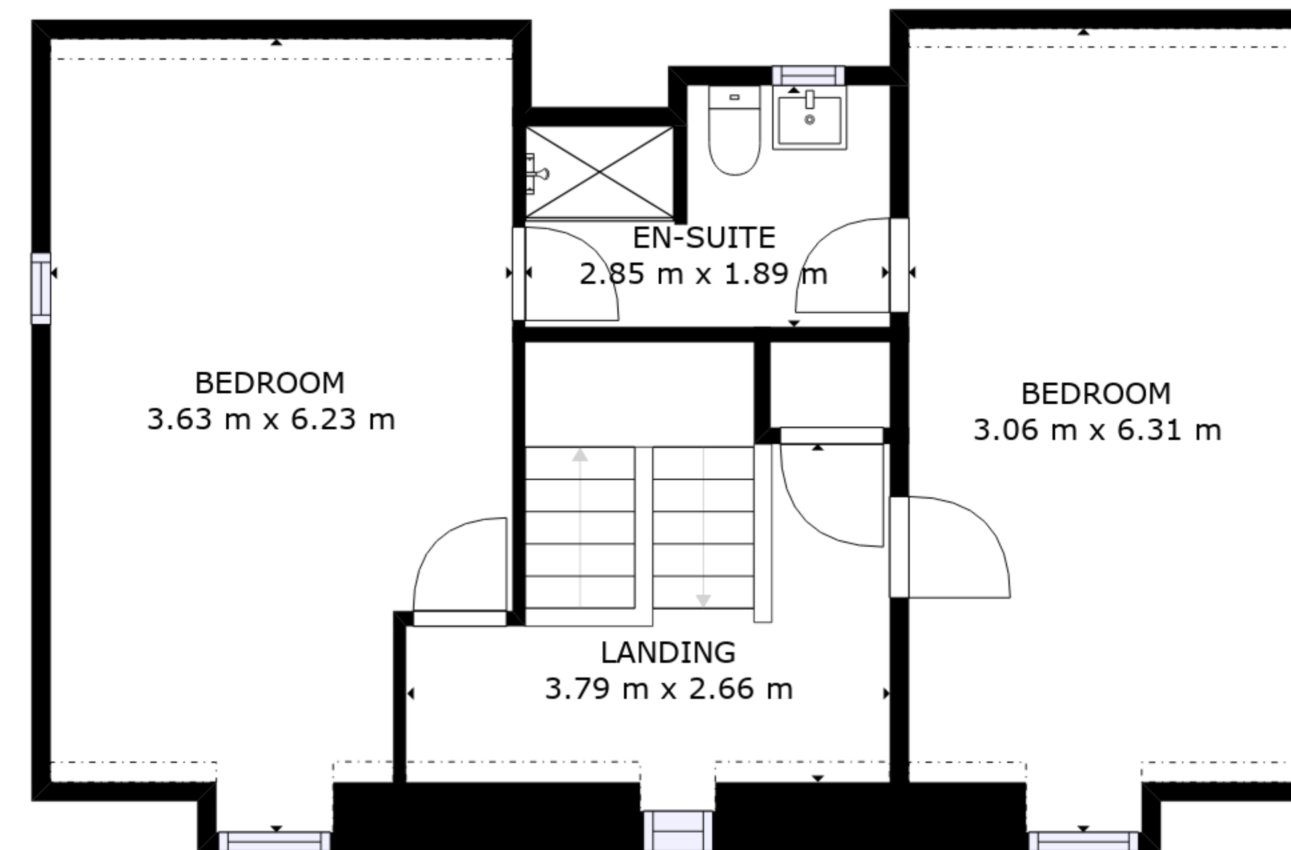
FLOOR 3
